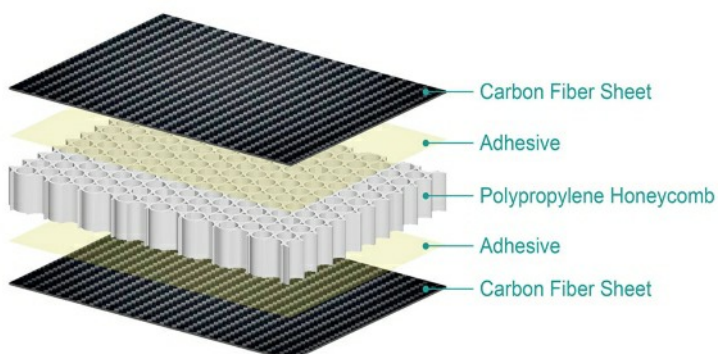
ONE PIECE HONEYCOMB FLOOR
